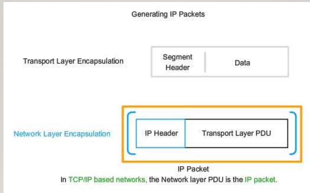
Figure 1: IP packet encapsulation from transport layer to network layer
